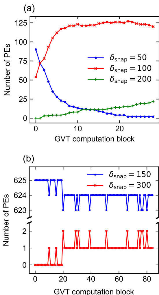
Fig. 8 Plots to illustrate the nature of dynamic updates to \delta_{snap} for (a) System 2 with lattice size 1200 \times 1200 and (b) System 4. In both cases, \Delta\tau_{GVT} = 120 s. For System 2, the number of PEs with the input \delta_{snap} value of 50 drops rapidly and irreversibly in the early stages of the simulation, reflecting the spatial homogeneity. In contrast, for System 4, most PEs preserve the input \delta_{snap} value of 150, while just one sparsifies irreversibly and others fluctuate between \delta_{snap} = 150 and \delta_{snap} = 300 .
